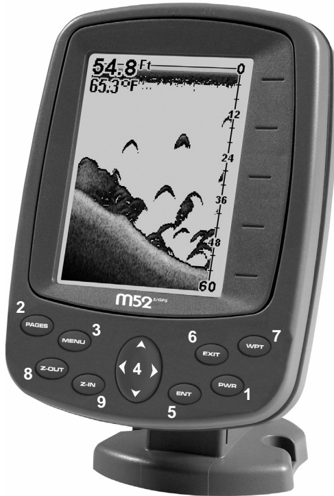
Lowrance M52 Sonar, front view, showing screen and keyboard. (A close-up of the keyboard can be found at the beginning of Sec. 6)
