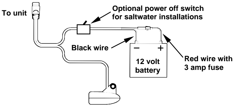
Power and transducer connections for the M52 sonar units (direct battery connection shown).
