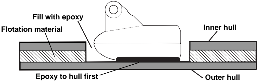
Epoxy the transducer to a solid portion of the hull.
