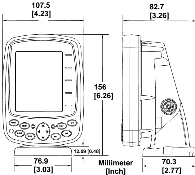
Front view (left) and side view (right) showing dimensions of the M52 when mounted on quick release bracket.
